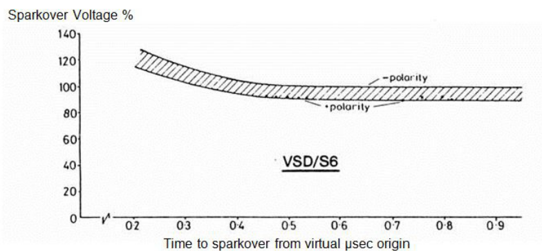
Figure 2 - Spark Over Voltage % of IEC 1.2/50 Wave 100% Spark Over Level
